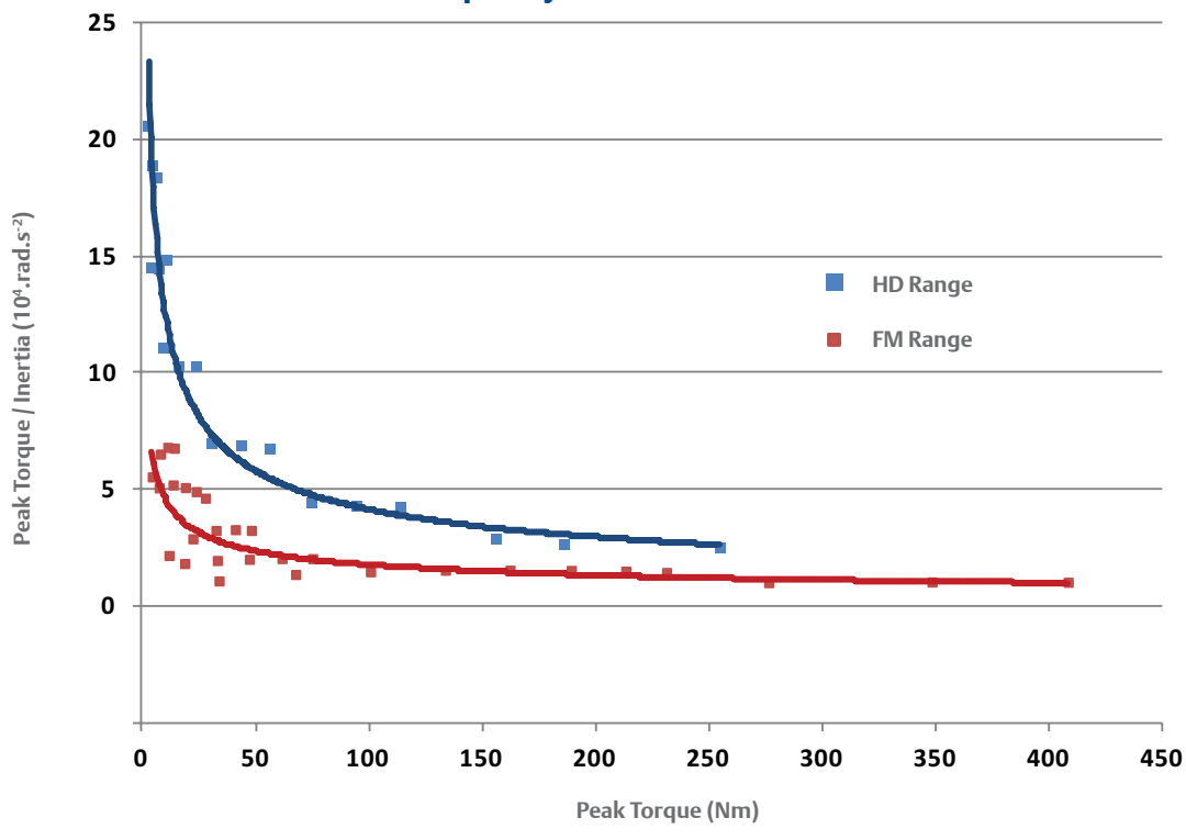
The Unimotor hd family ranges from 55 mm to 190 mm
